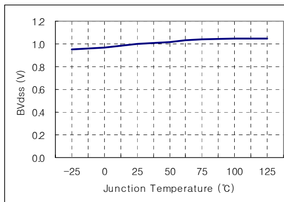
Breakdown Voltage vs. Temp
