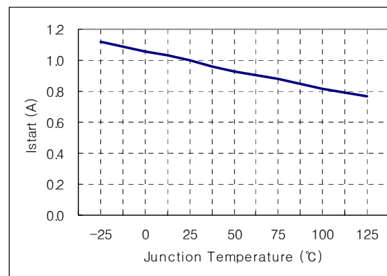
Start Up Current vs. Temp (for FSD200)
