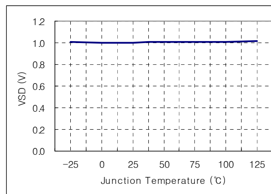
Shutdown Feedback Voltage vs. Temp
