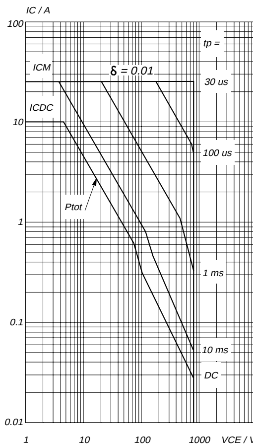
Fig.16. Forward bias safe operating area. T_{hs} = 25^\circ C I_{CD} & I_{CM} = f(V_{CE}) ; I_{CM} single pulse; parameter t_p Second-breakdown limits independent of temperature. Mounted with heatsink compound.
