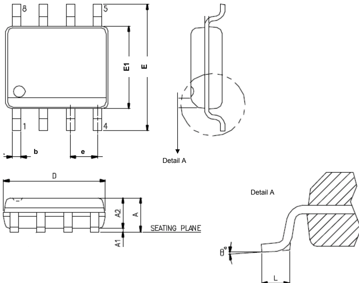
Figure 26. SOP 8 ( 150 mil )
