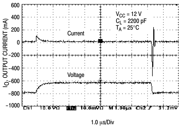
Figure 6. Output Waveform
