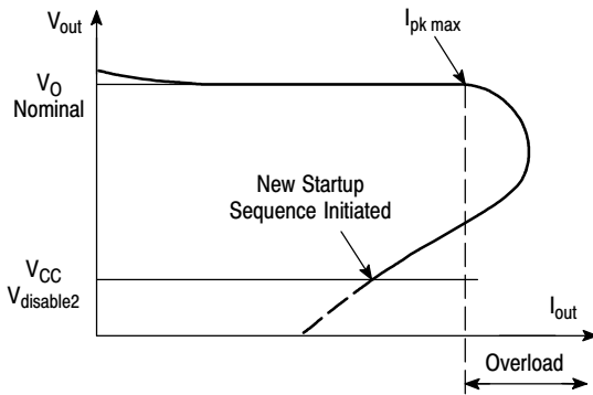
Figure 46. Foldback Characteristic
