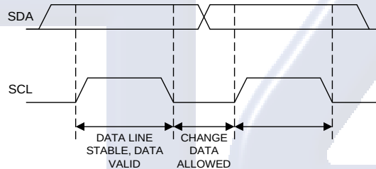
Fig. 17 Data Validity on the I 2 C BUS
