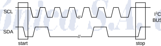
Fig. 18 Timing diagram of I 2 C BUS
