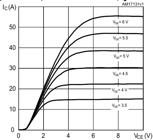
Figure 7. Output characteristics ( T_J = -40\text{ °C} )
